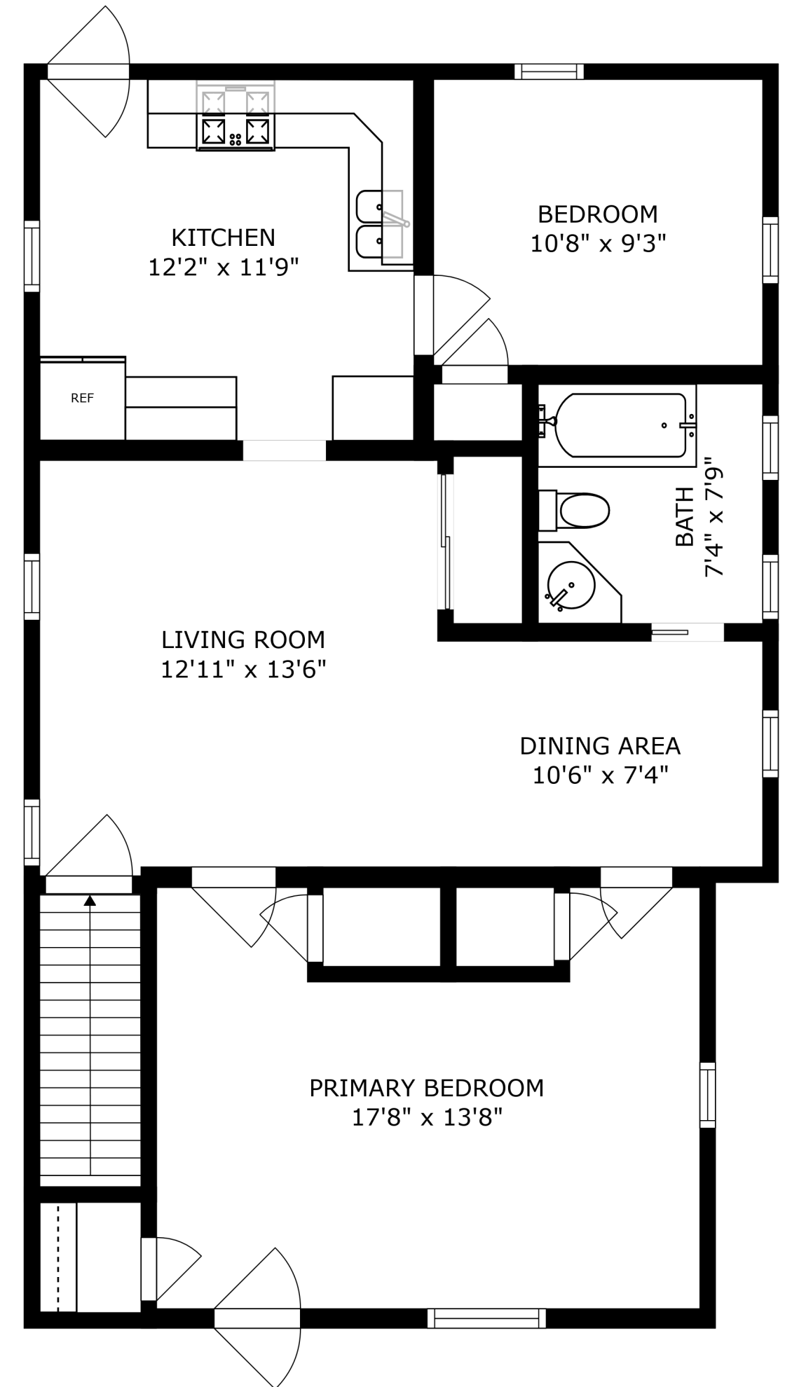
FLOOR 3
