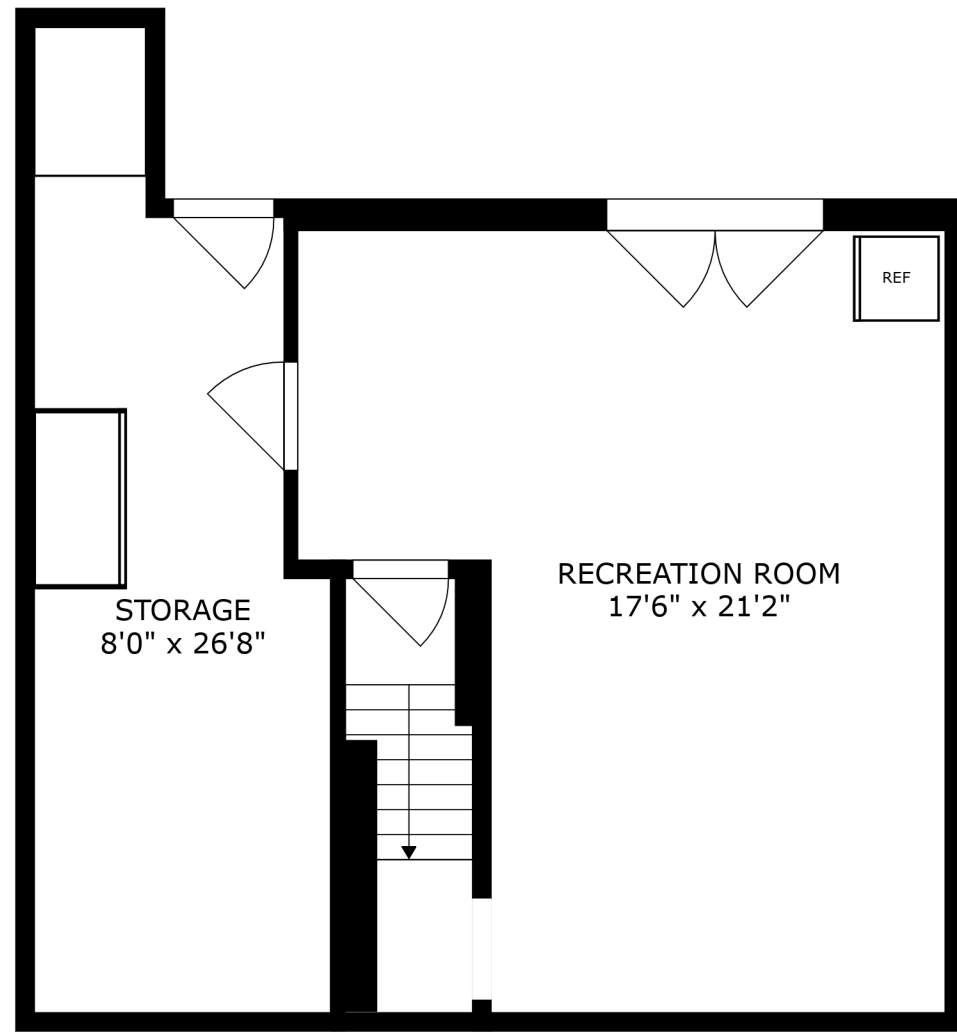
FLOOR 1
