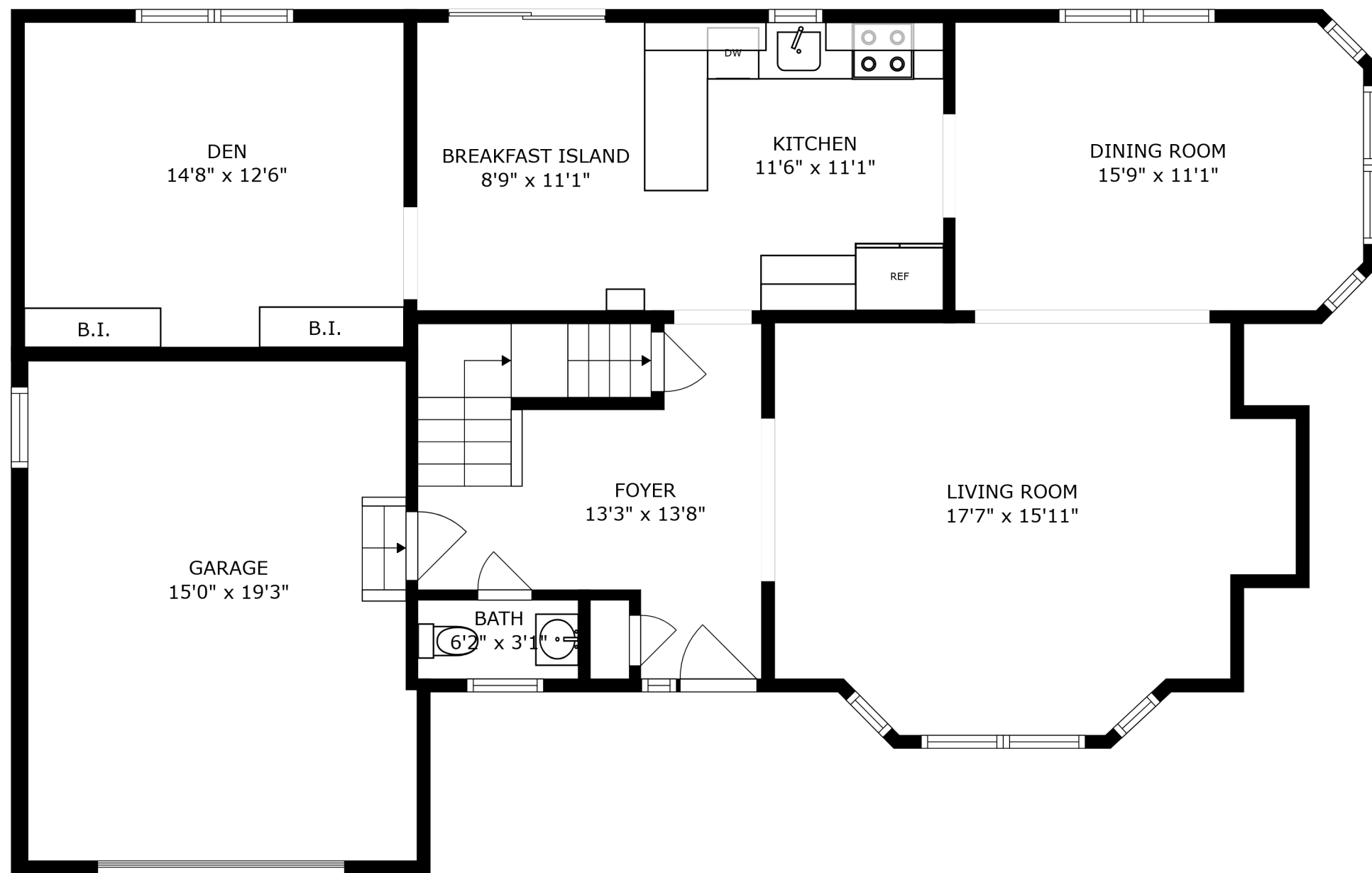
FLOOR 2
