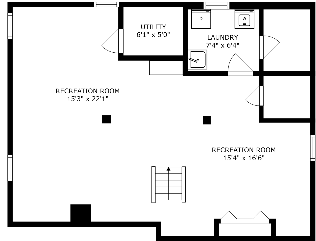
FLOOR 1
