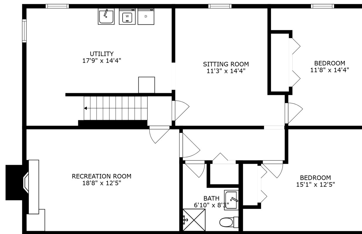
FLOOR 1
