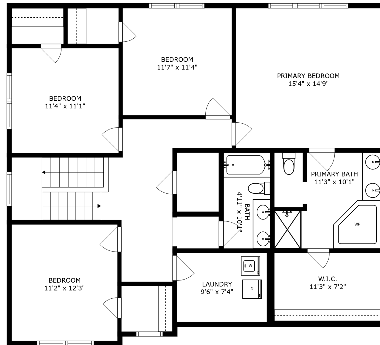
FLOOR 3
