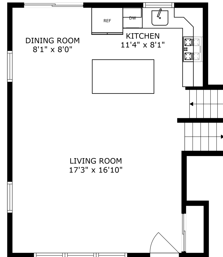
FLOOR 2
