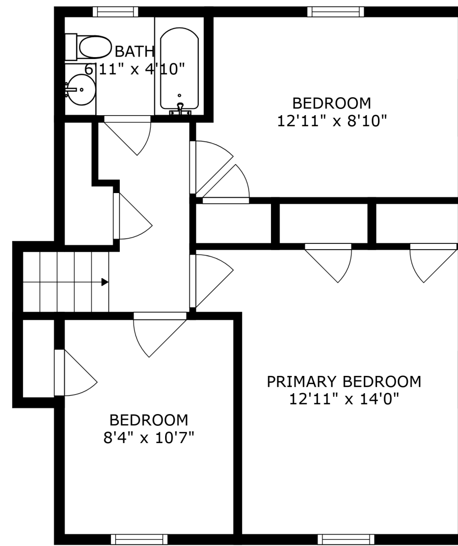
FLOOR 3
