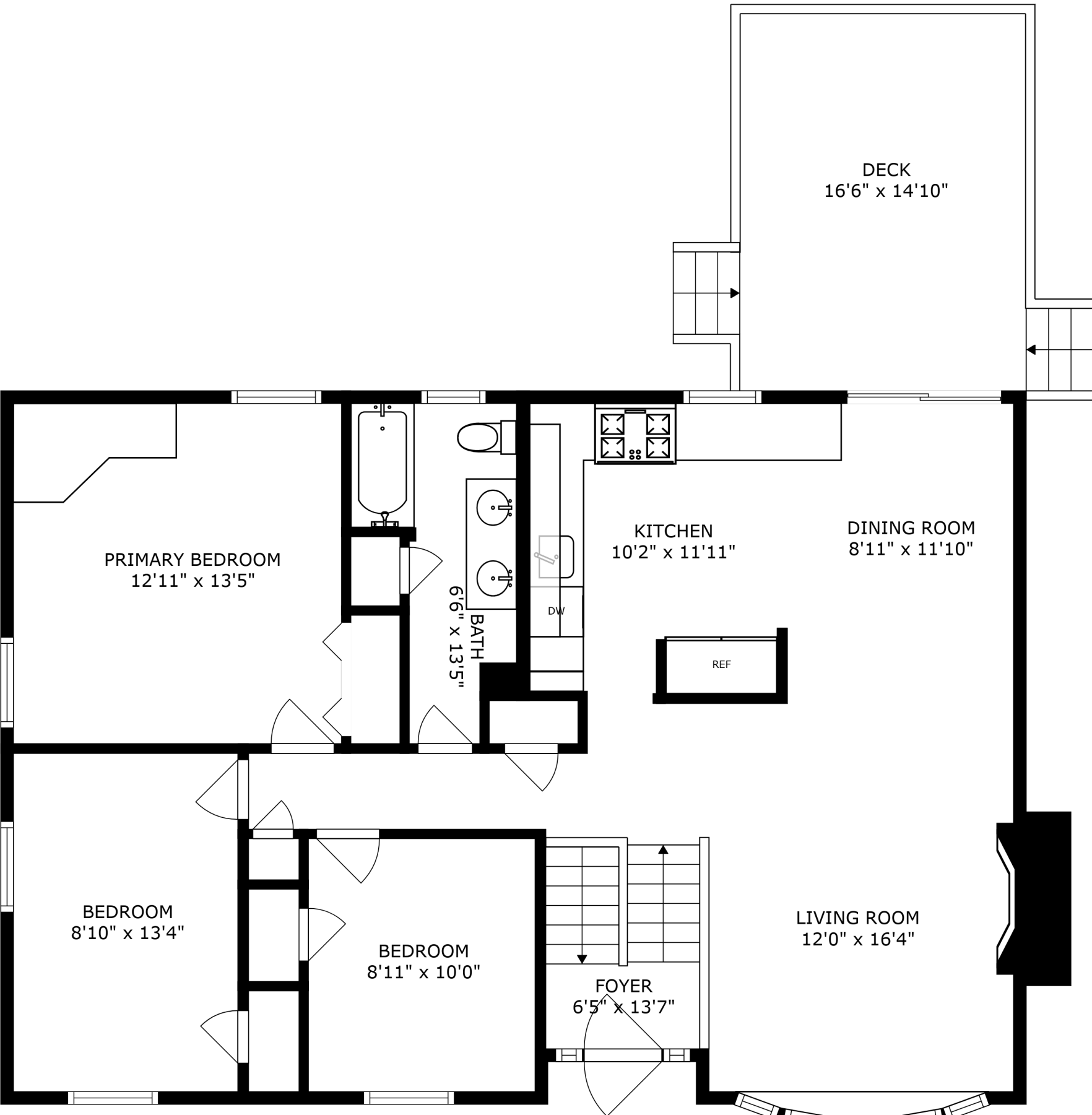
FLOOR 2
