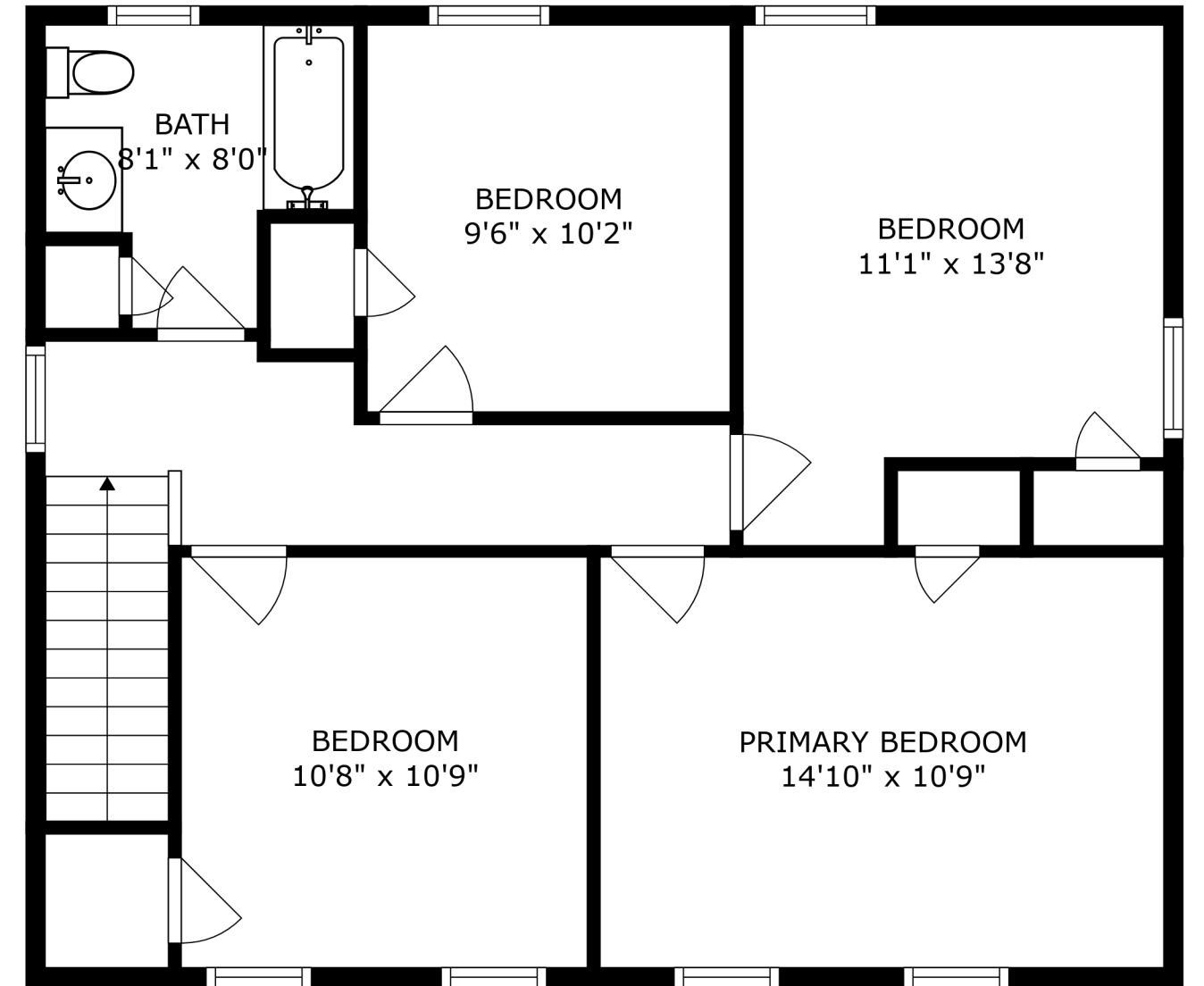
FLOOR 2
