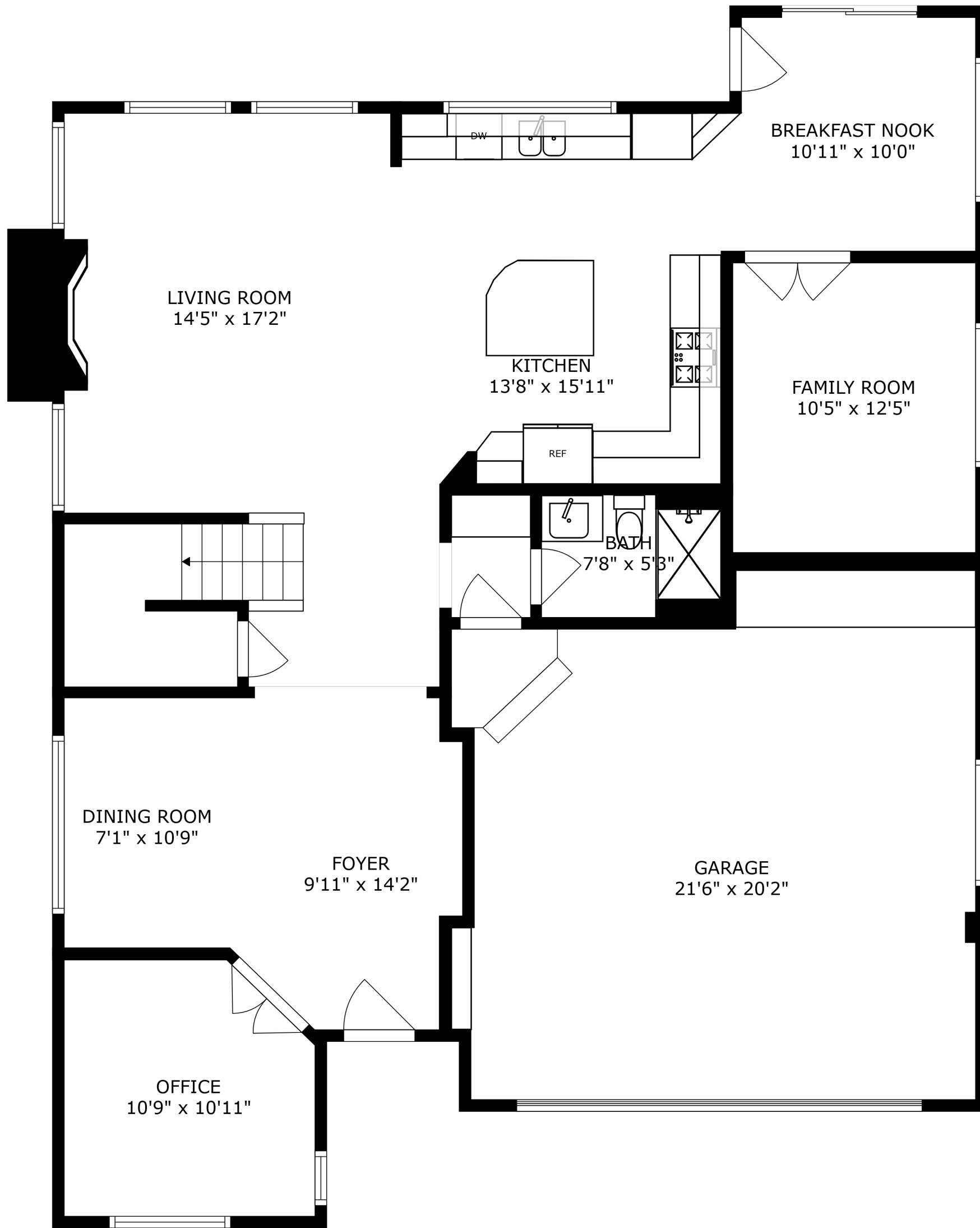
FLOOR 1
