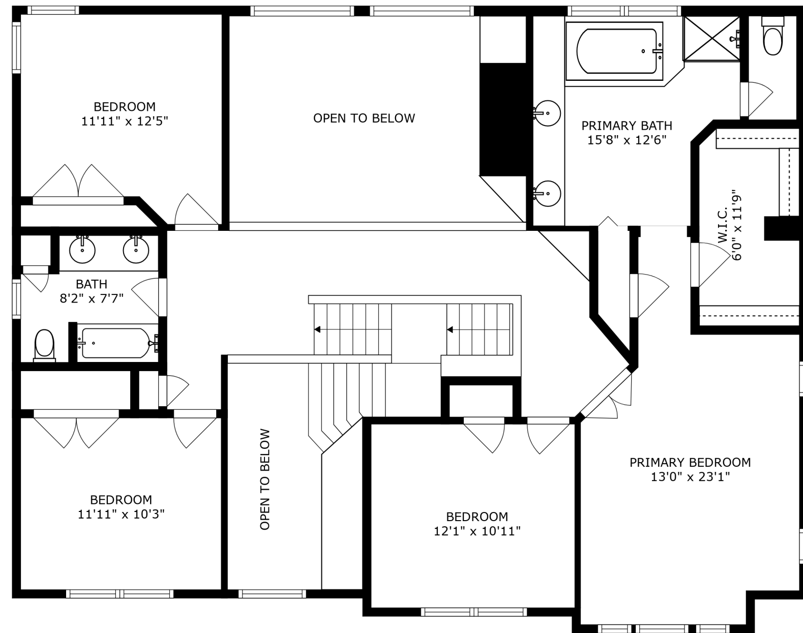
FLOOR 3
