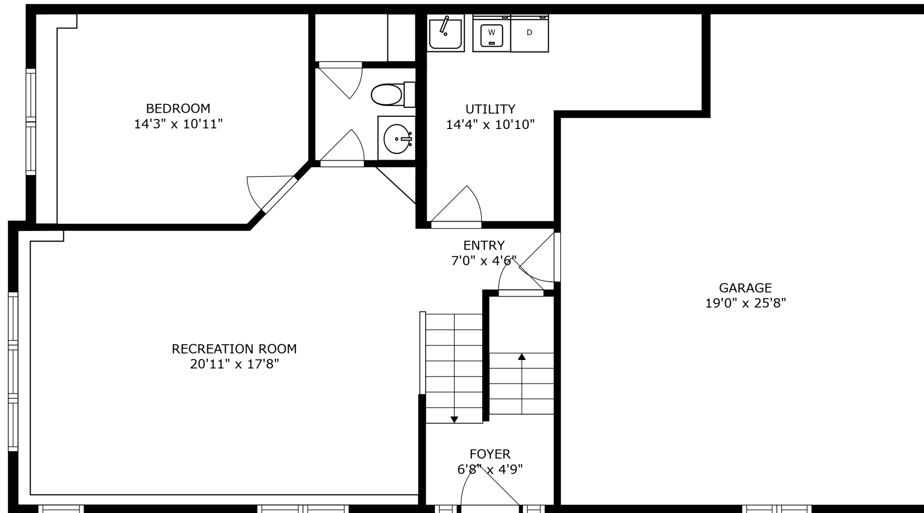
FLOOR 1
