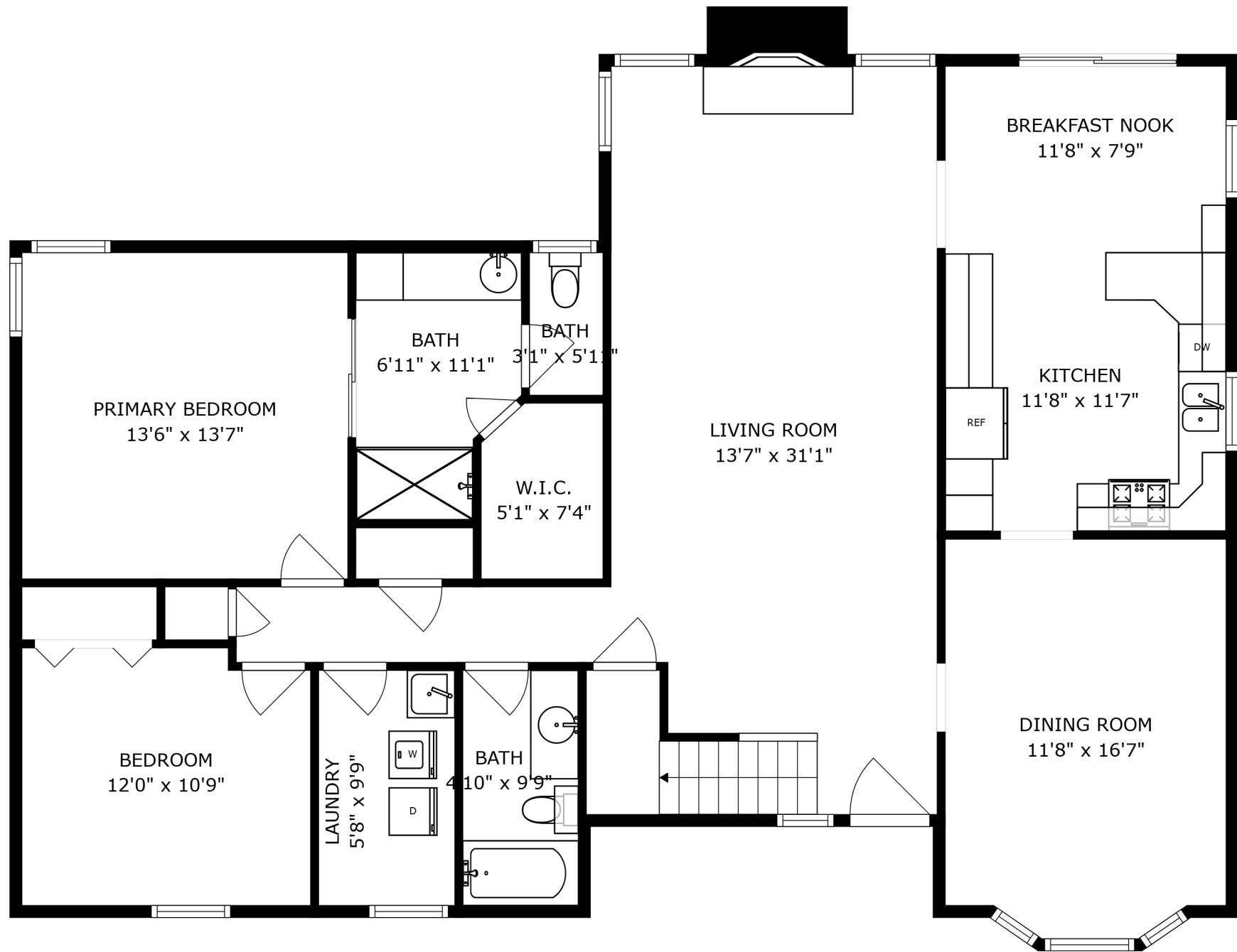
FLOOR 1
