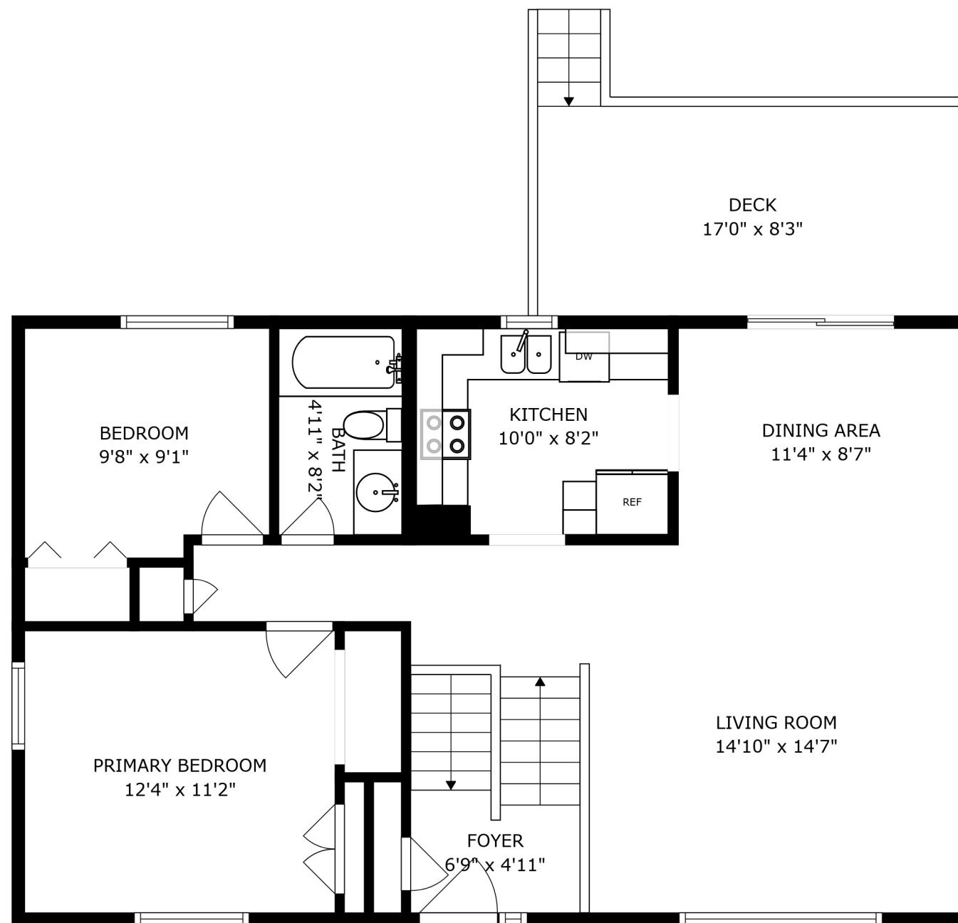
FLOOR 2
