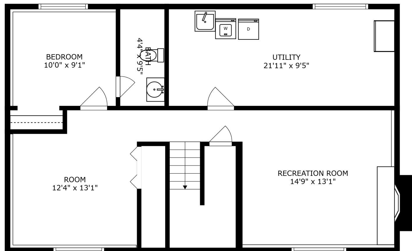
FLOOR 2
