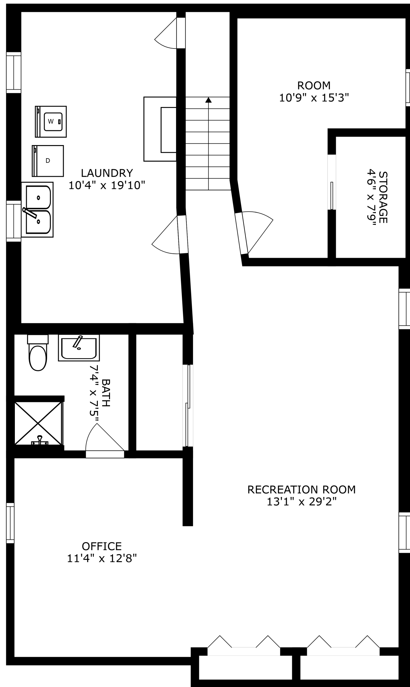
FLOOR 1
