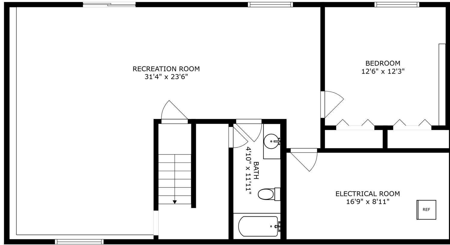
FLOOR 1
