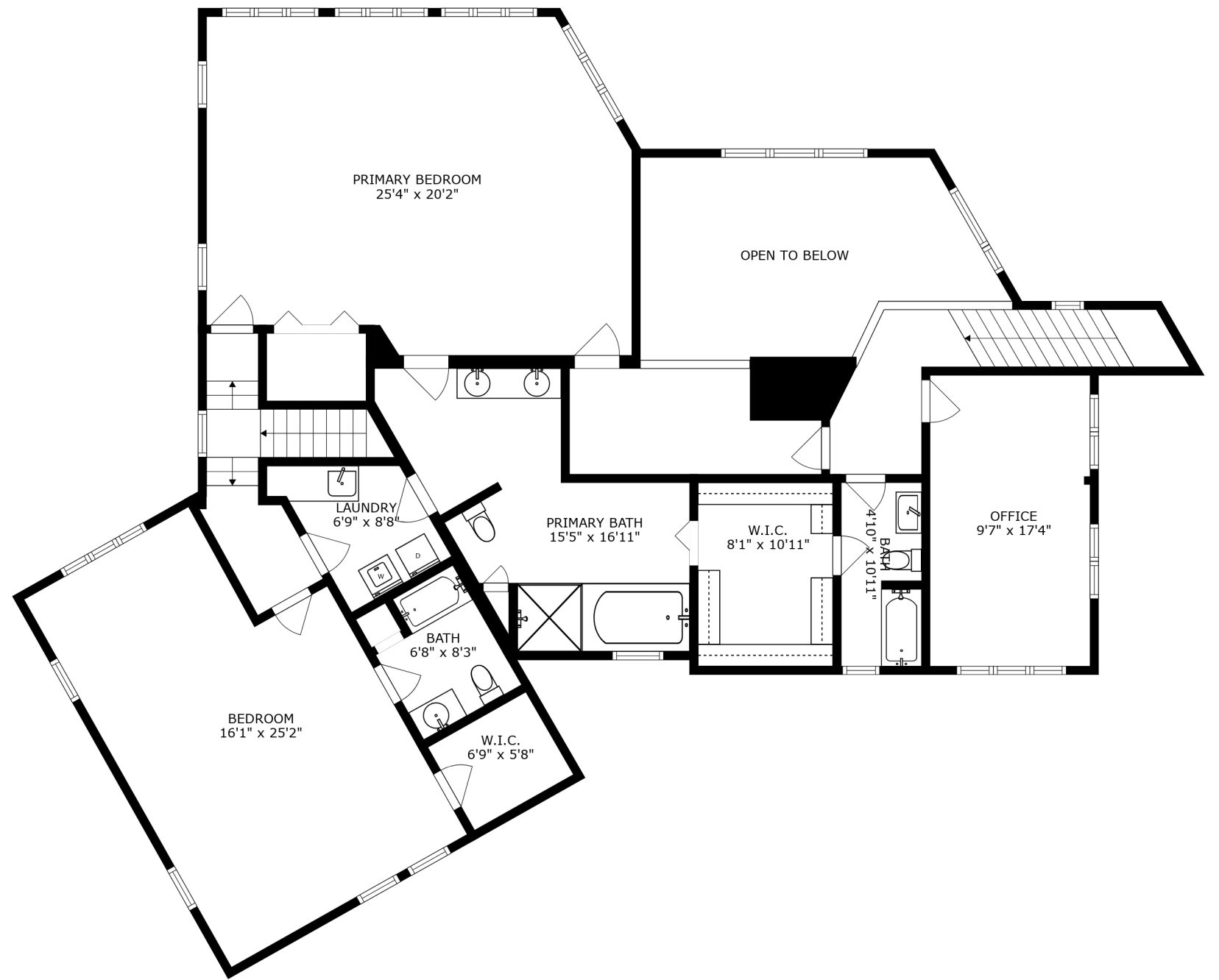
FLOOR 3
