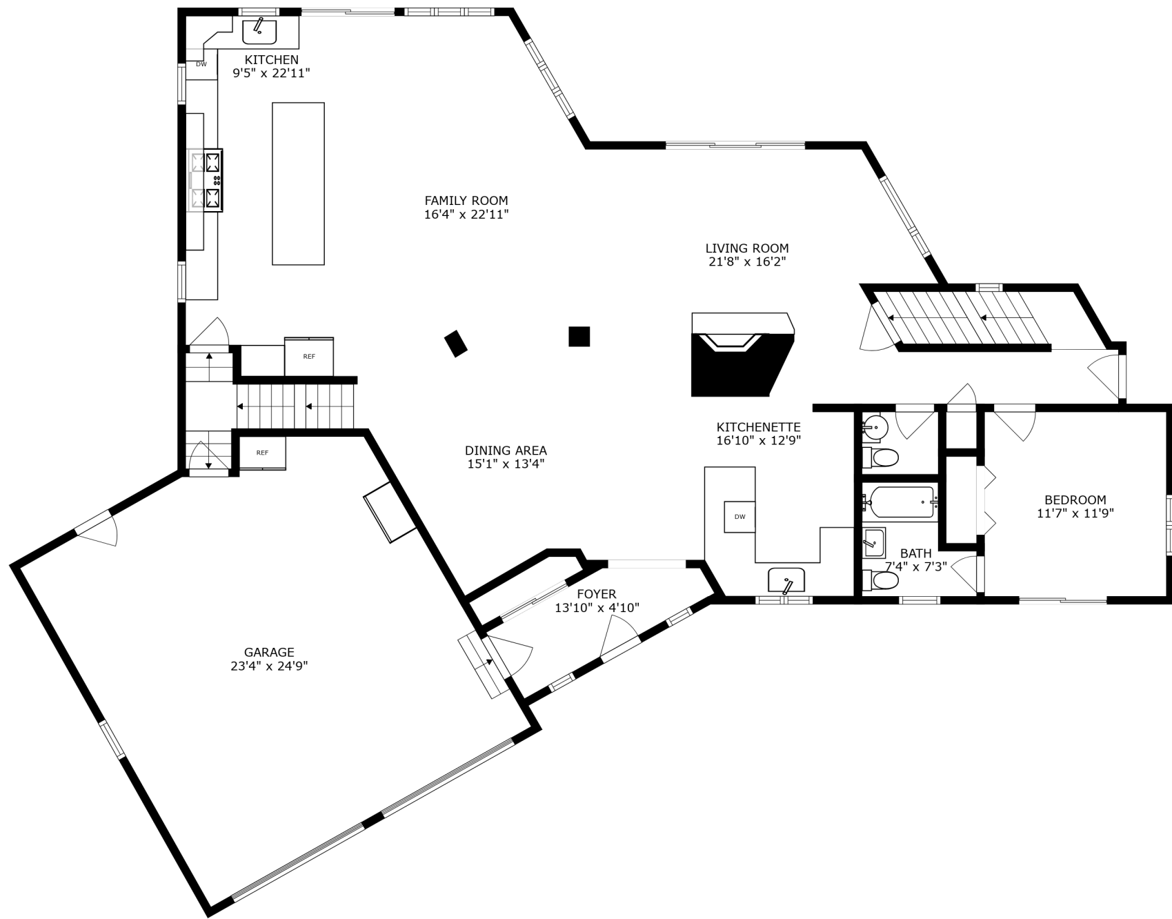
FLOOR 2
