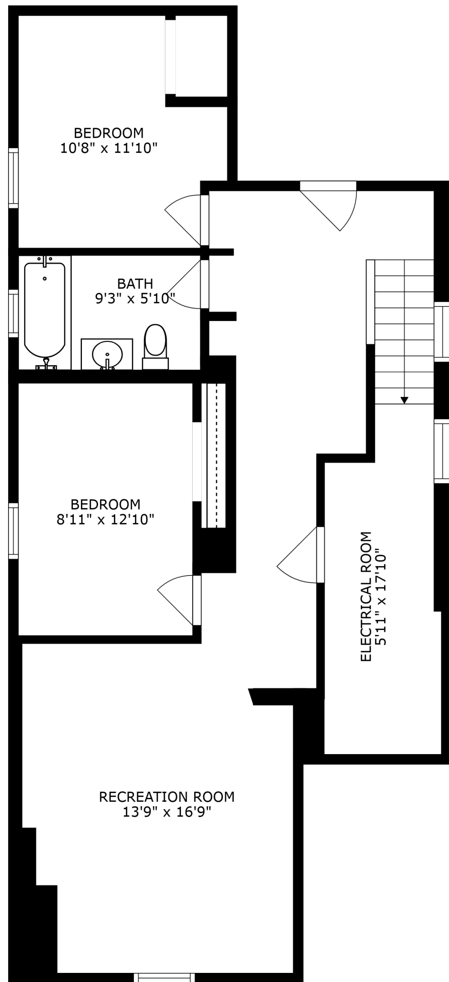
FLOOR 1
