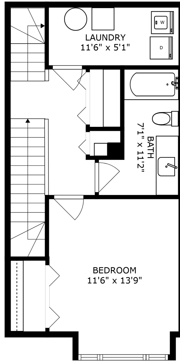
FLOOR 3
