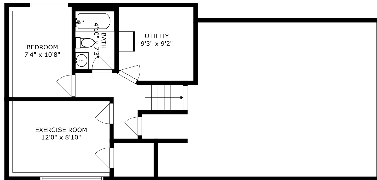
FLOOR 2
