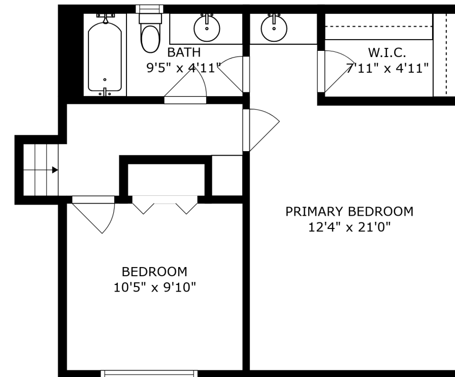
FLOOR 4
