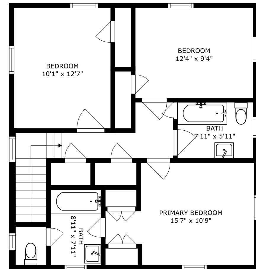
FLOOR 3
