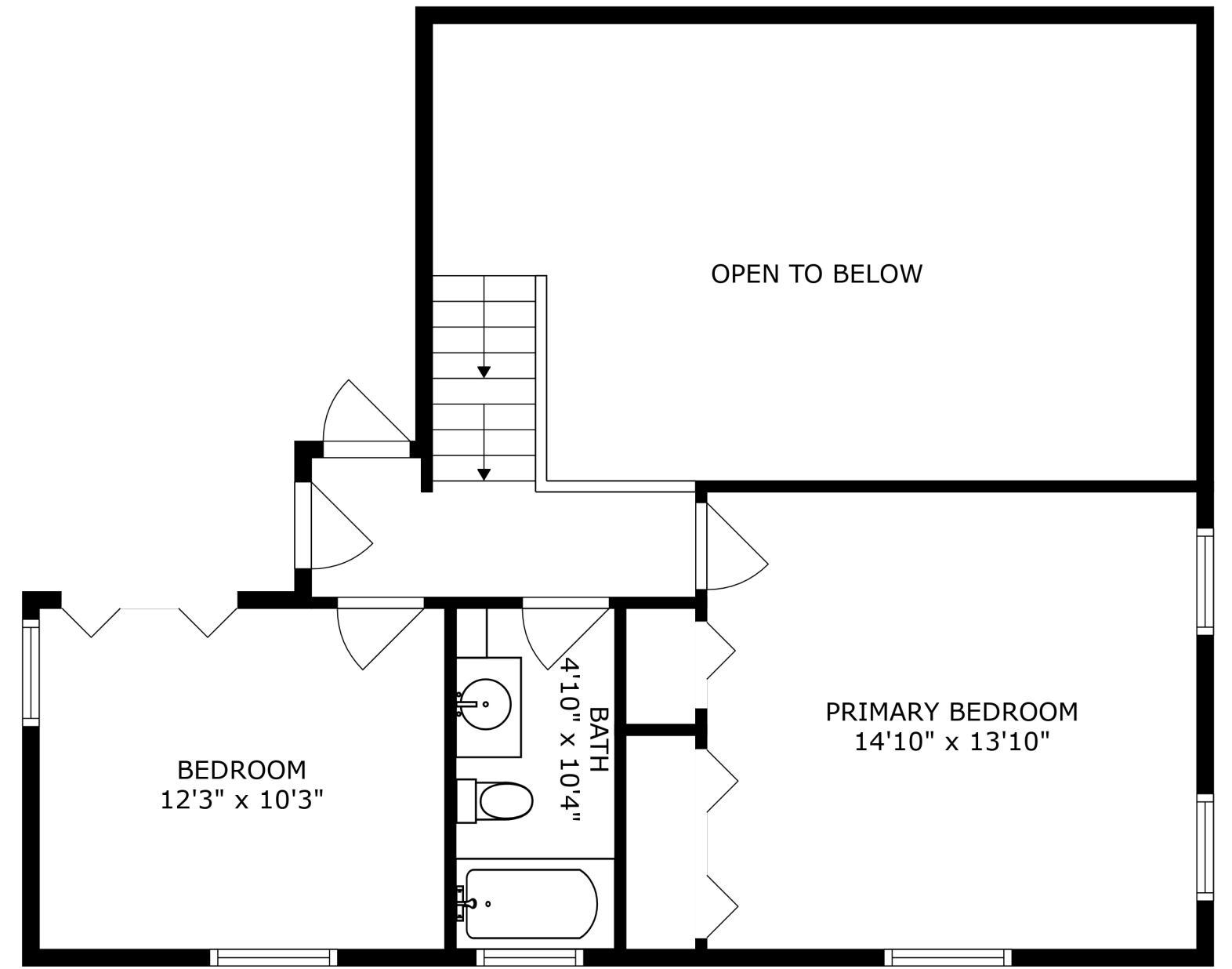
FLOOR 3
