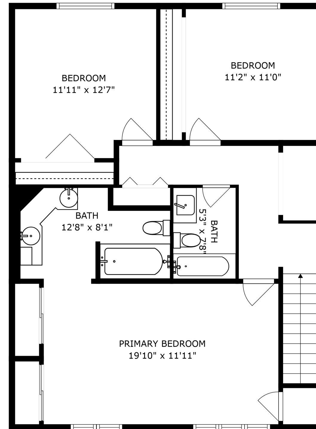
FLOOR 2
