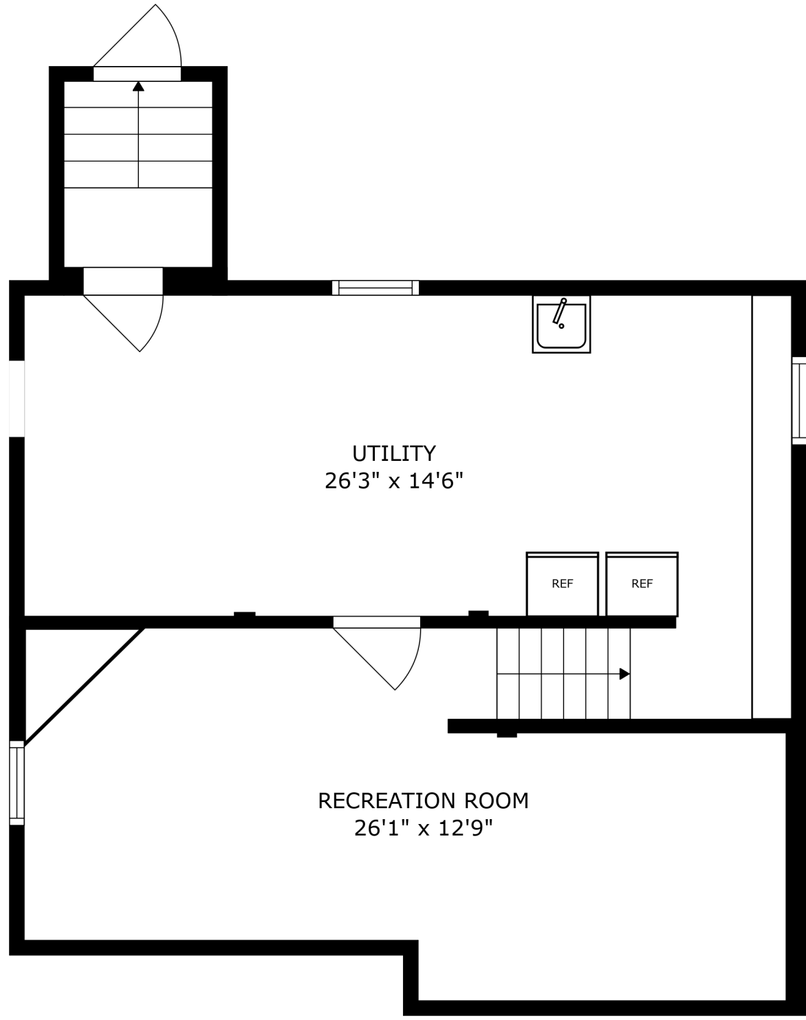
FLOOR 1
