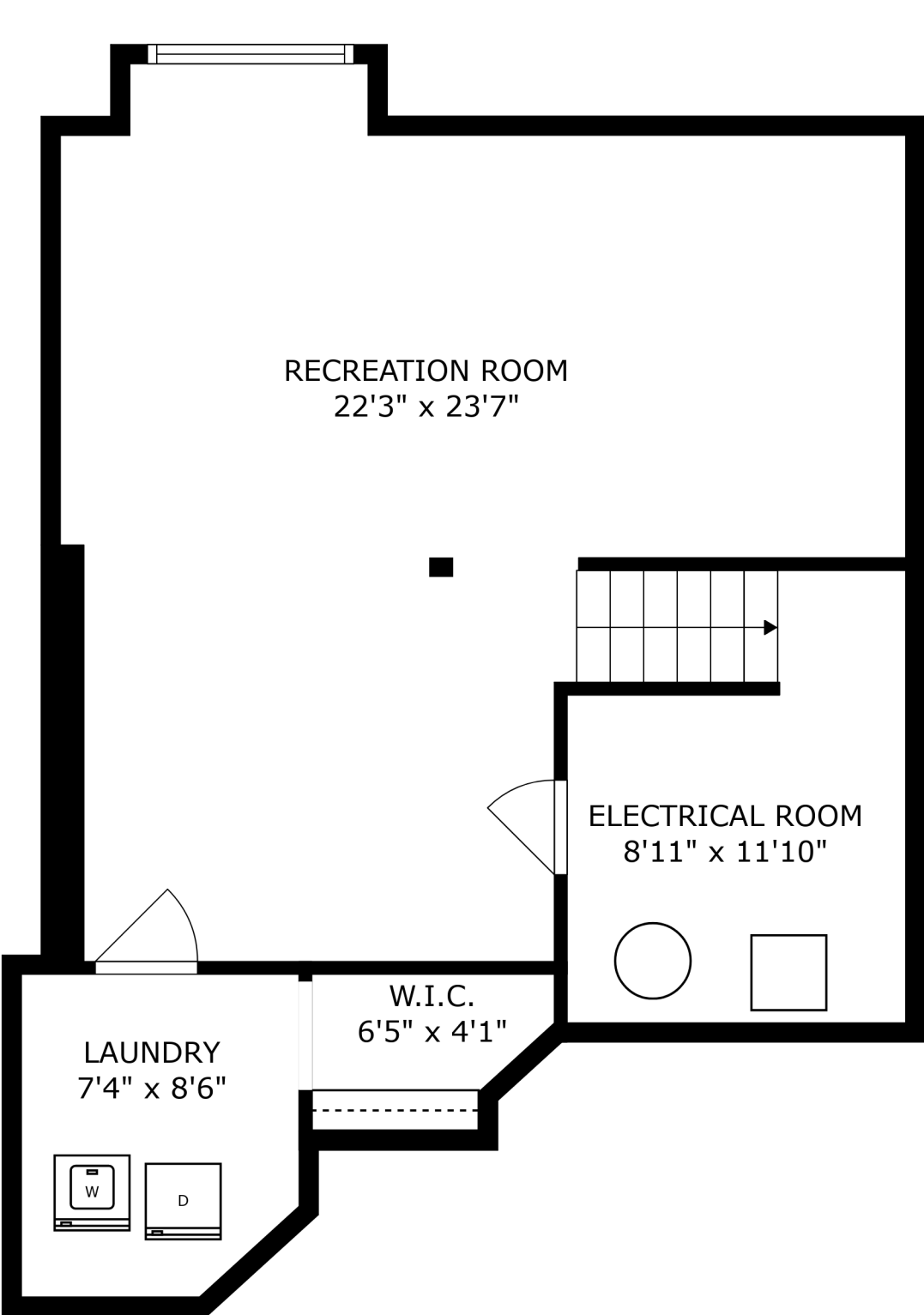
FLOOR 1
