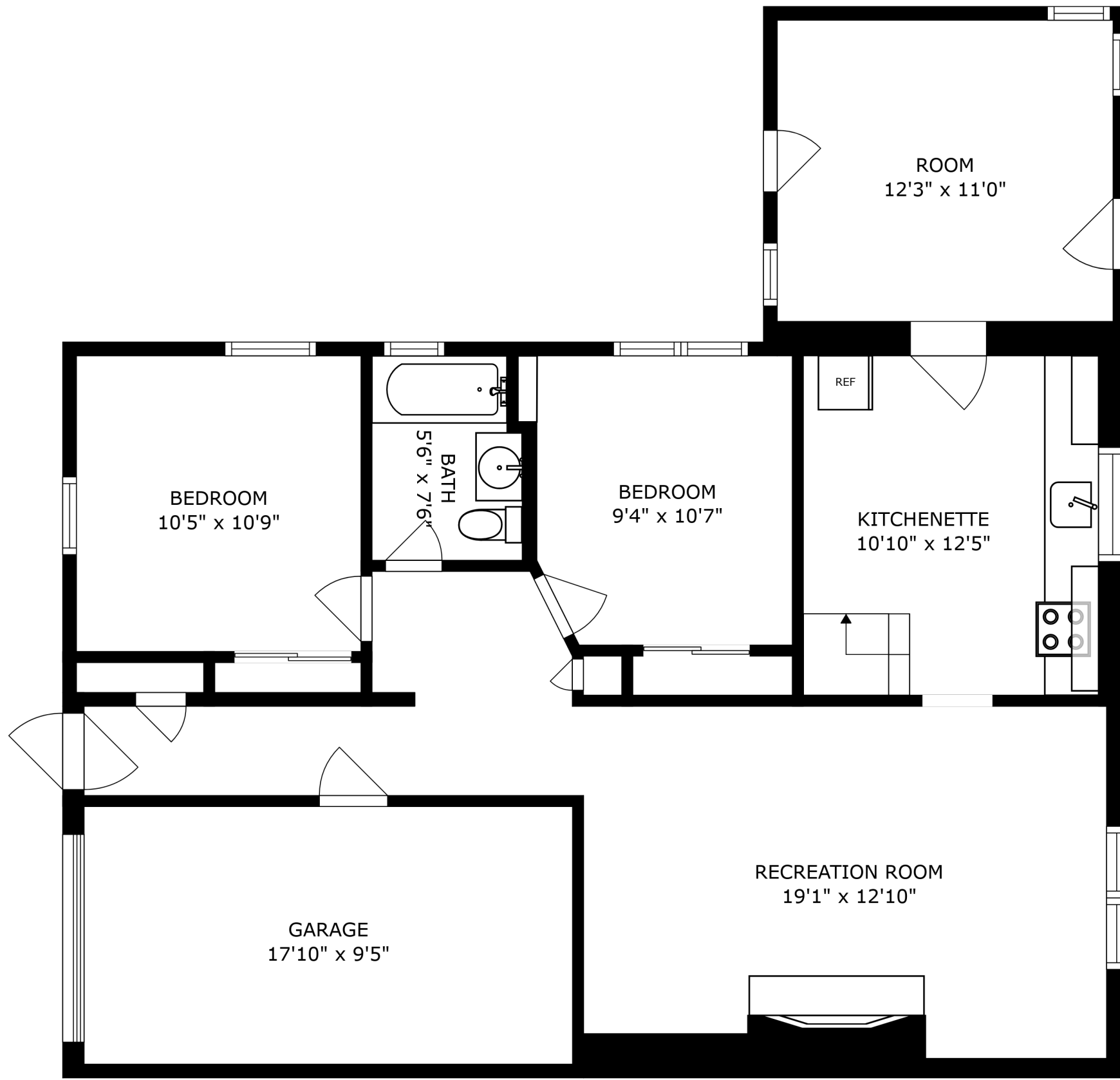
FLOOR 1
