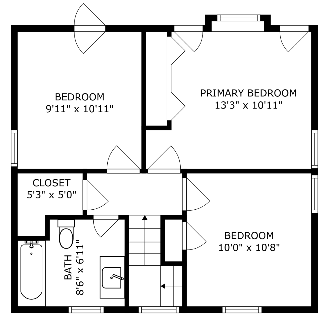
FLOOR 2
