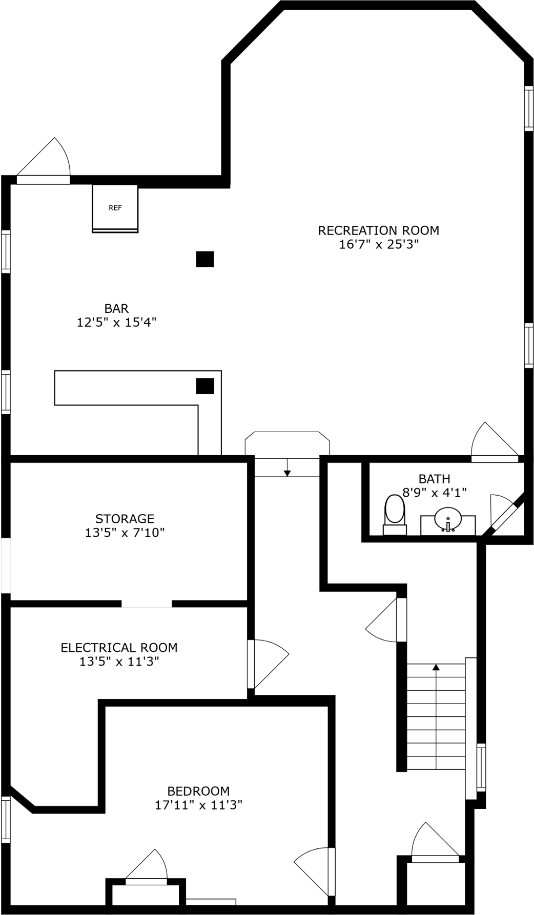
FLOOR 1
