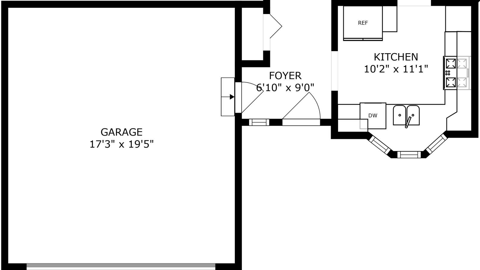
FLOOR 2
