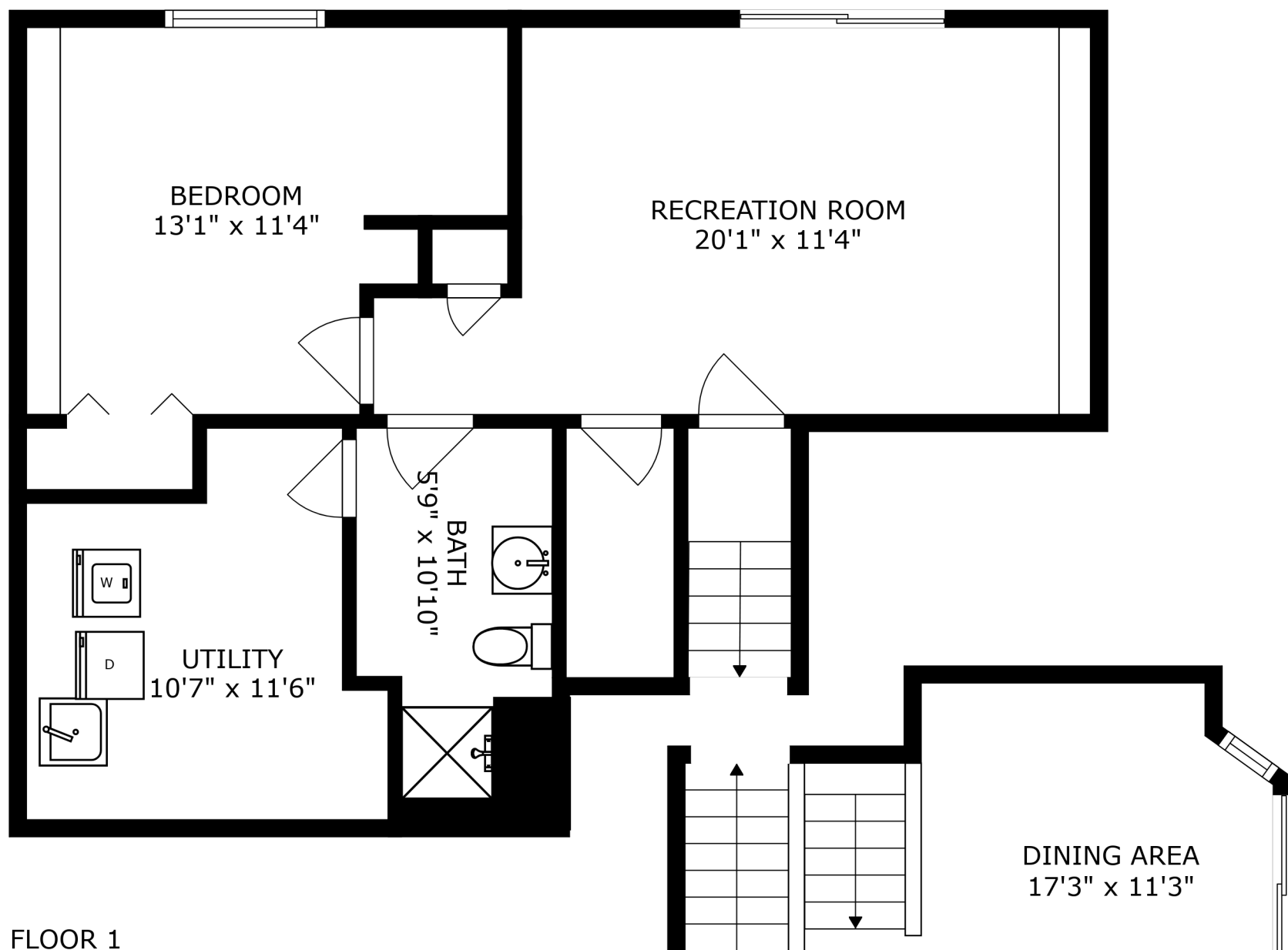
FLOOR 1
