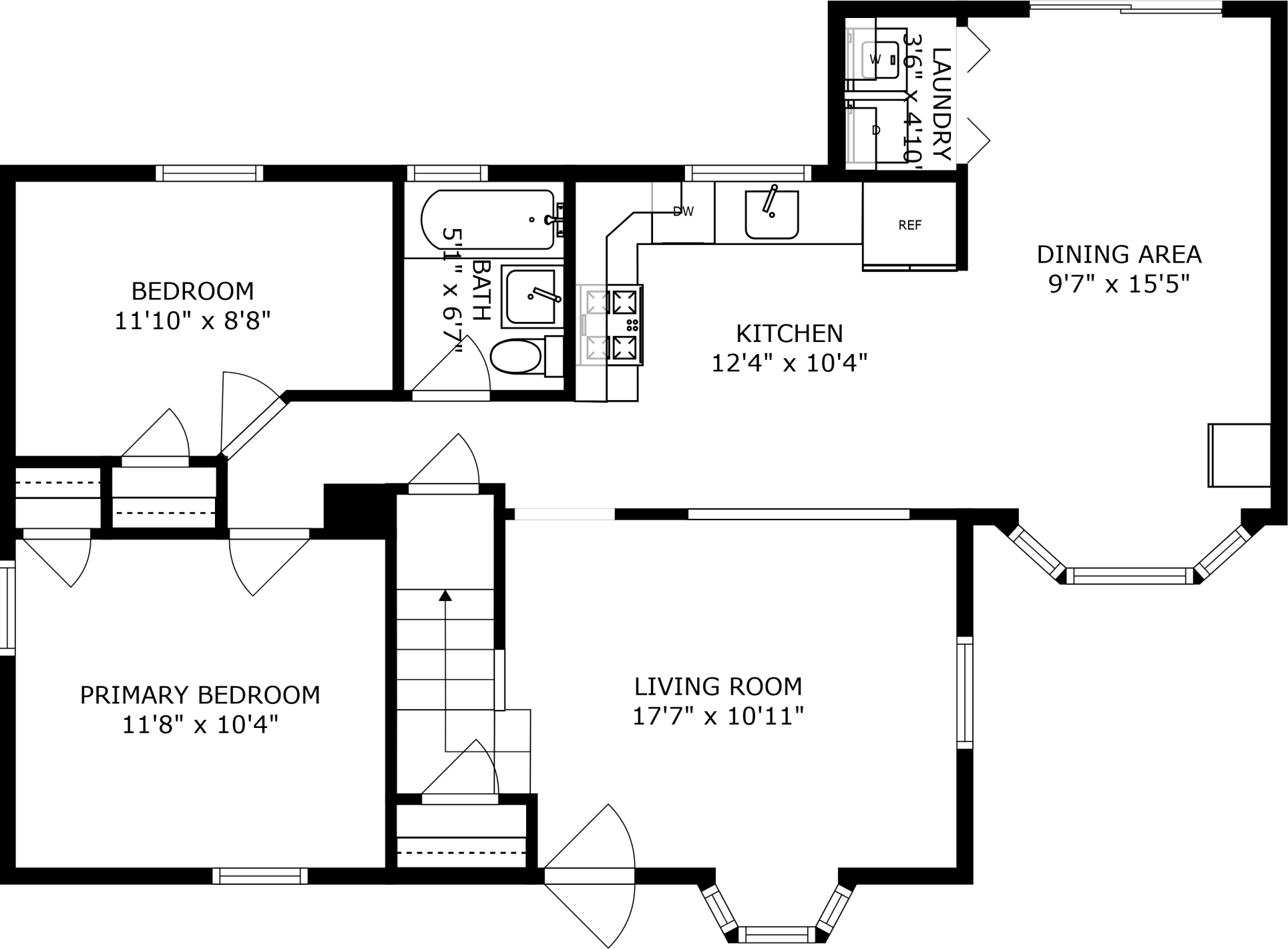
FLOOR 1
