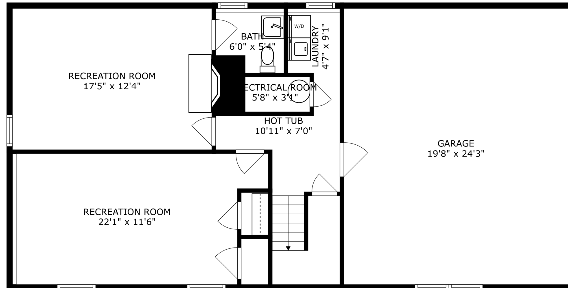
FLOOR 1
