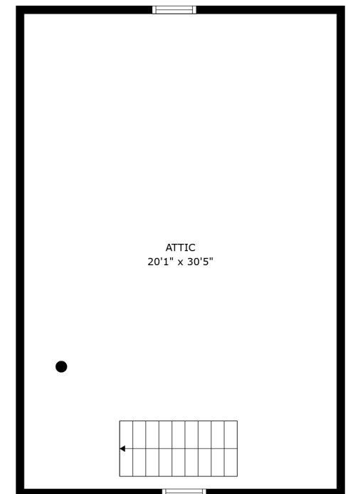
FLOOR 6
