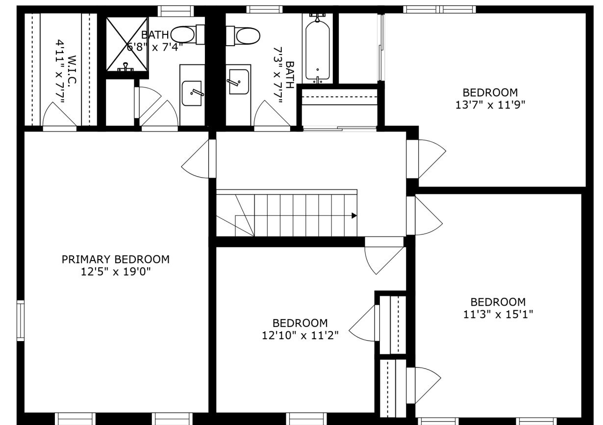
FLOOR 3
