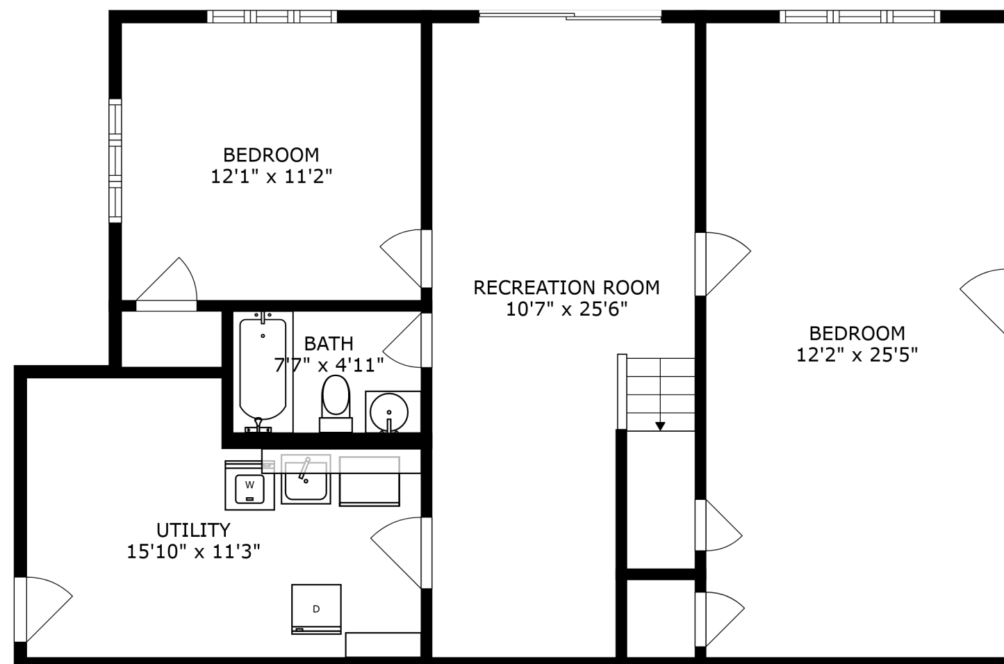
FLOOR 2
