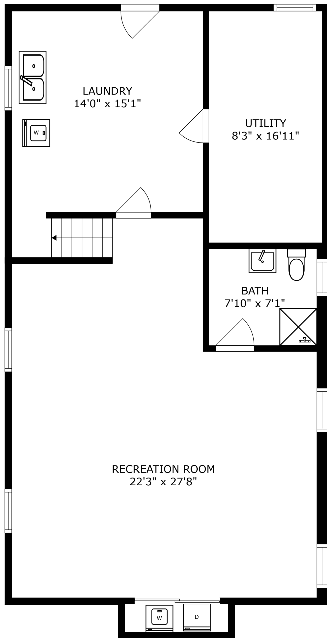
FLOOR 1
