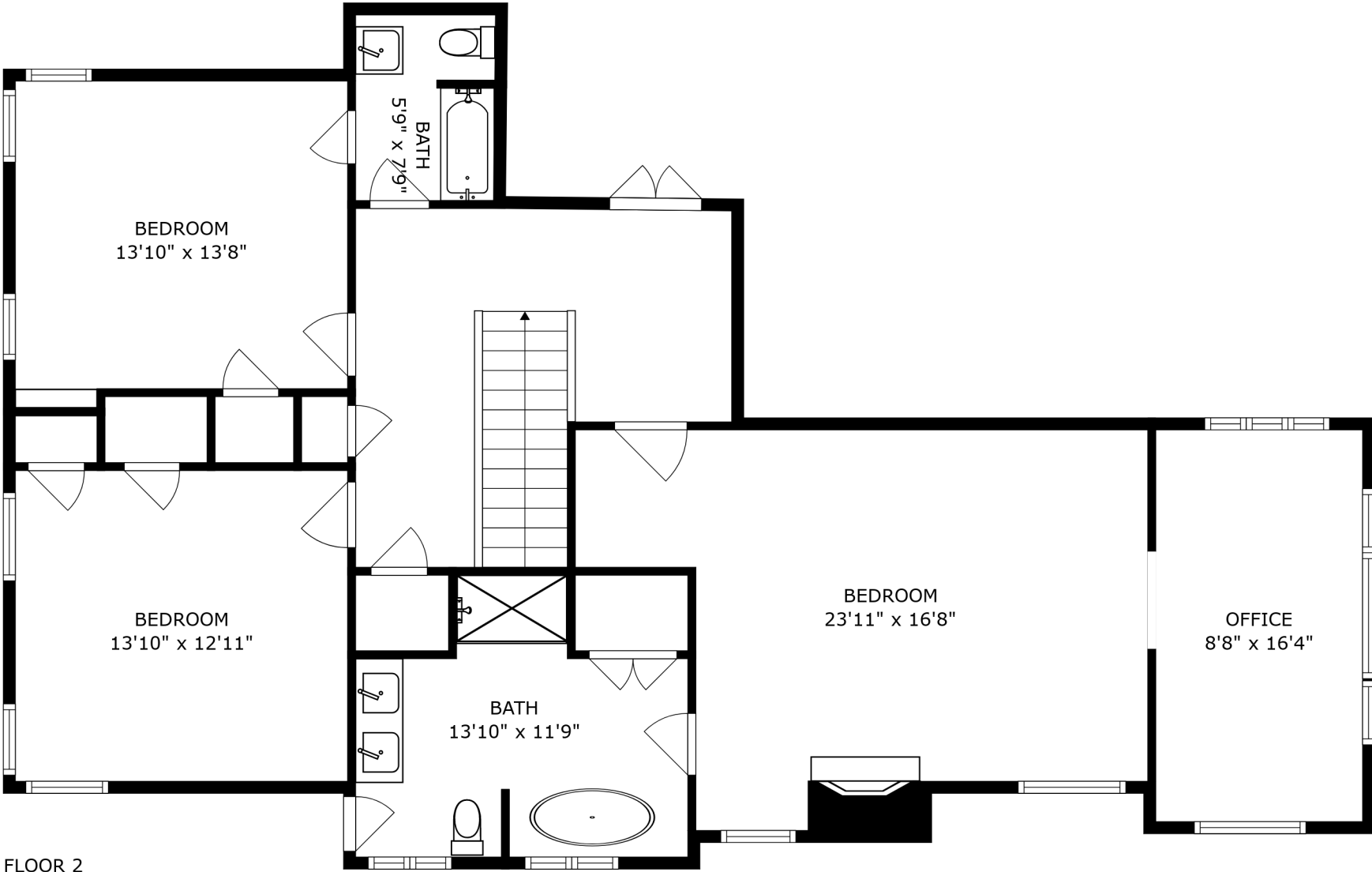
FLOOR 2
