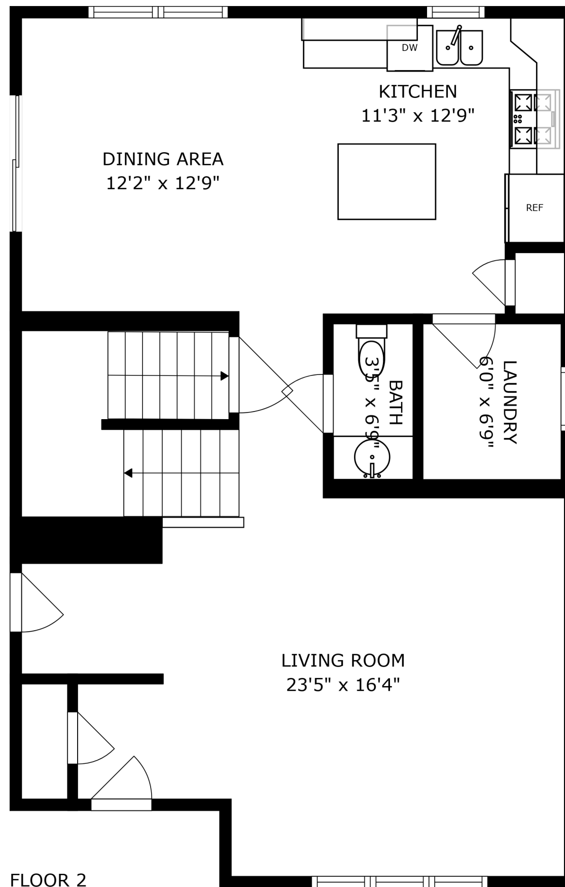
FLOOR 2
