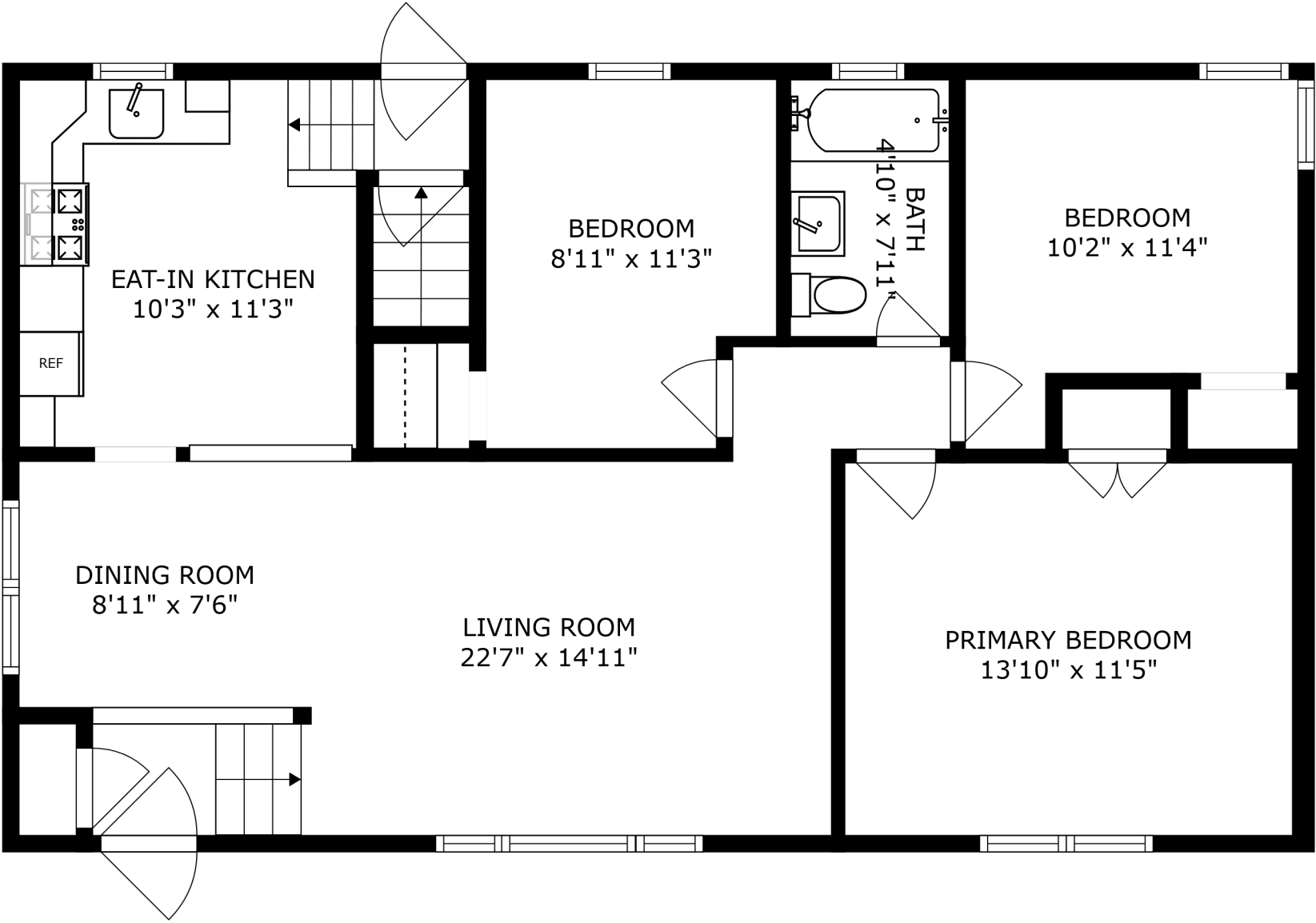
FLOOR 2
