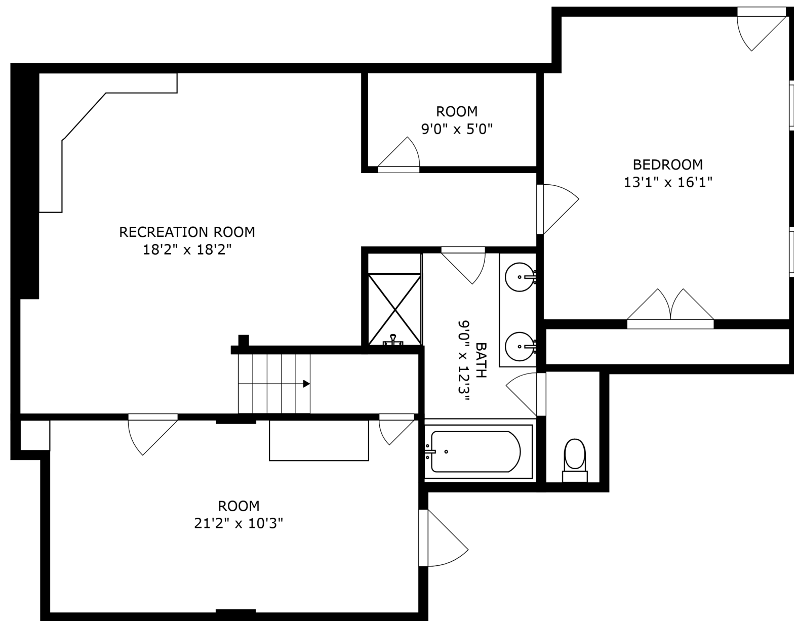
FLOOR 1
