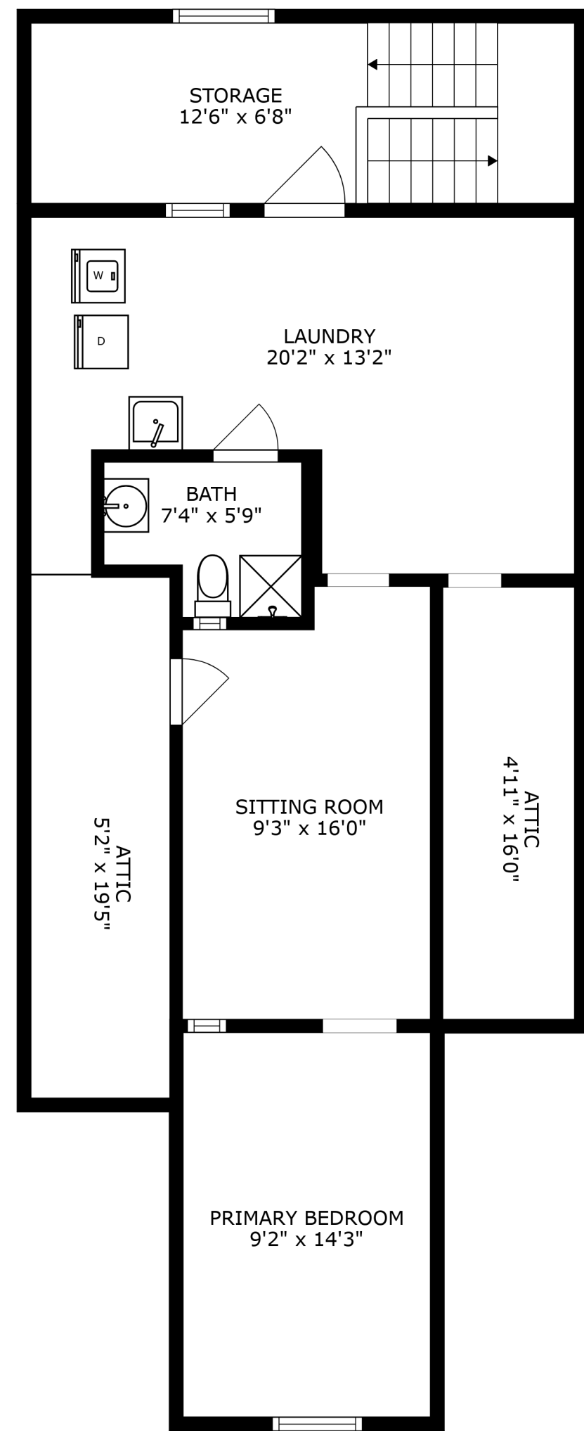
FLOOR 3
