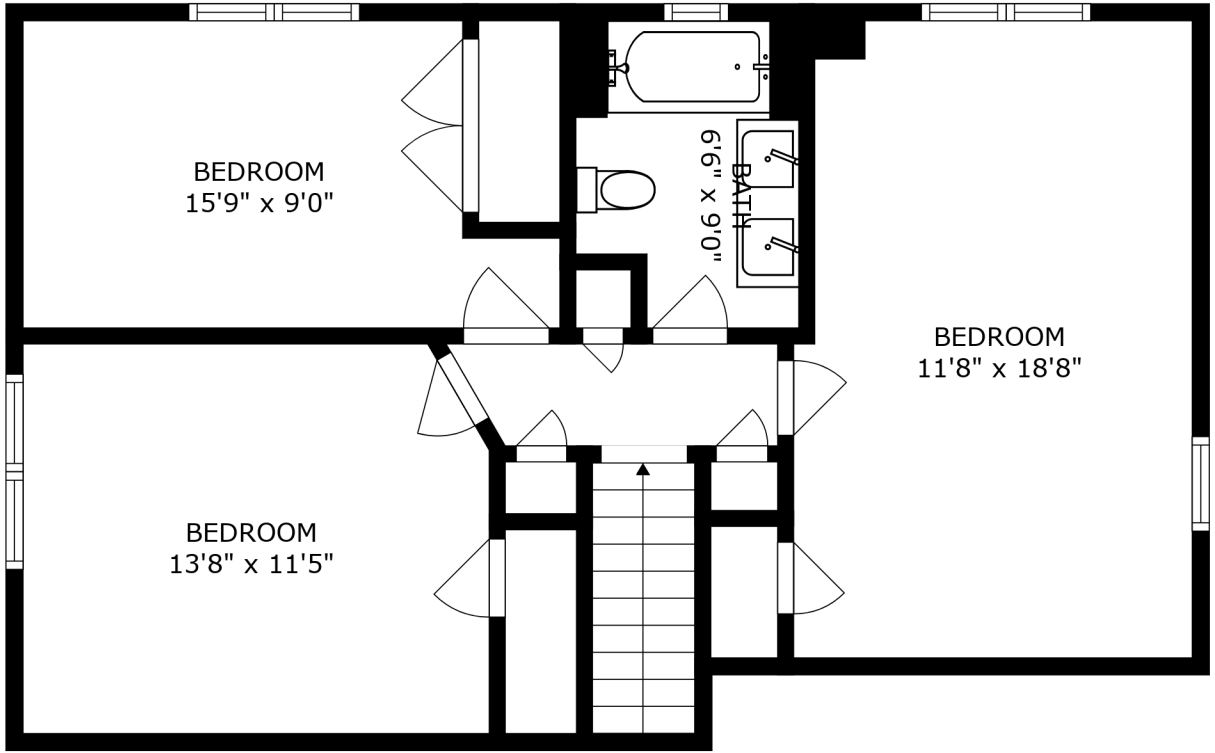
FLOOR 3
