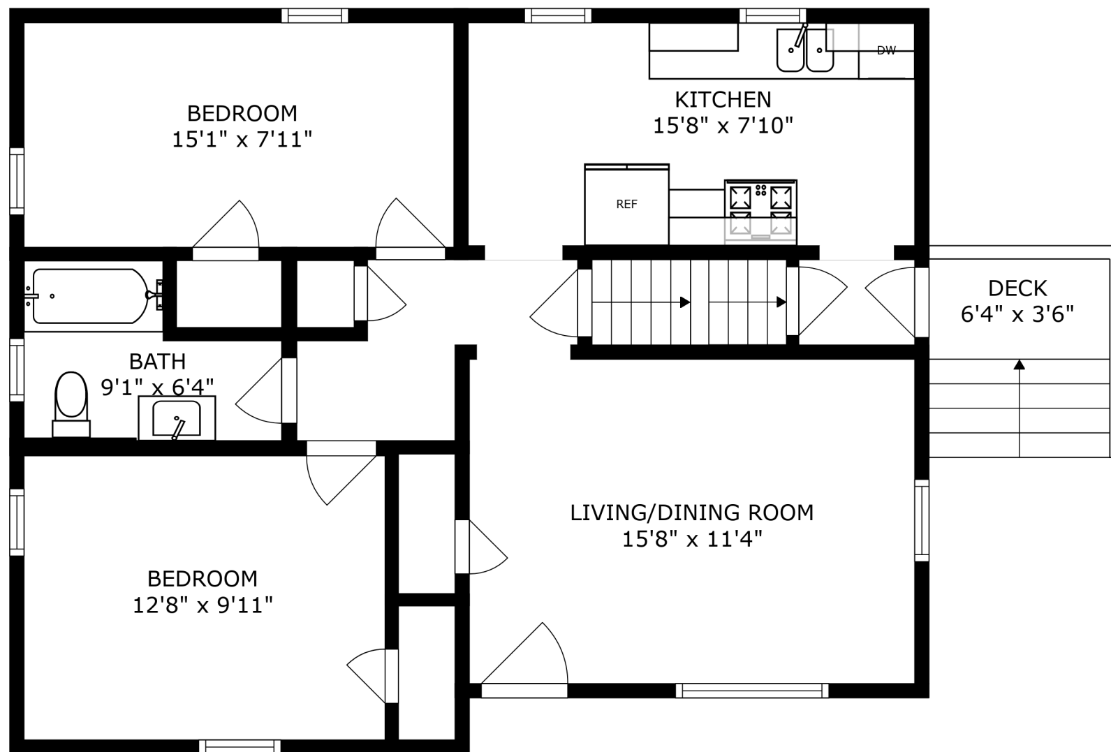
FLOOR 2
