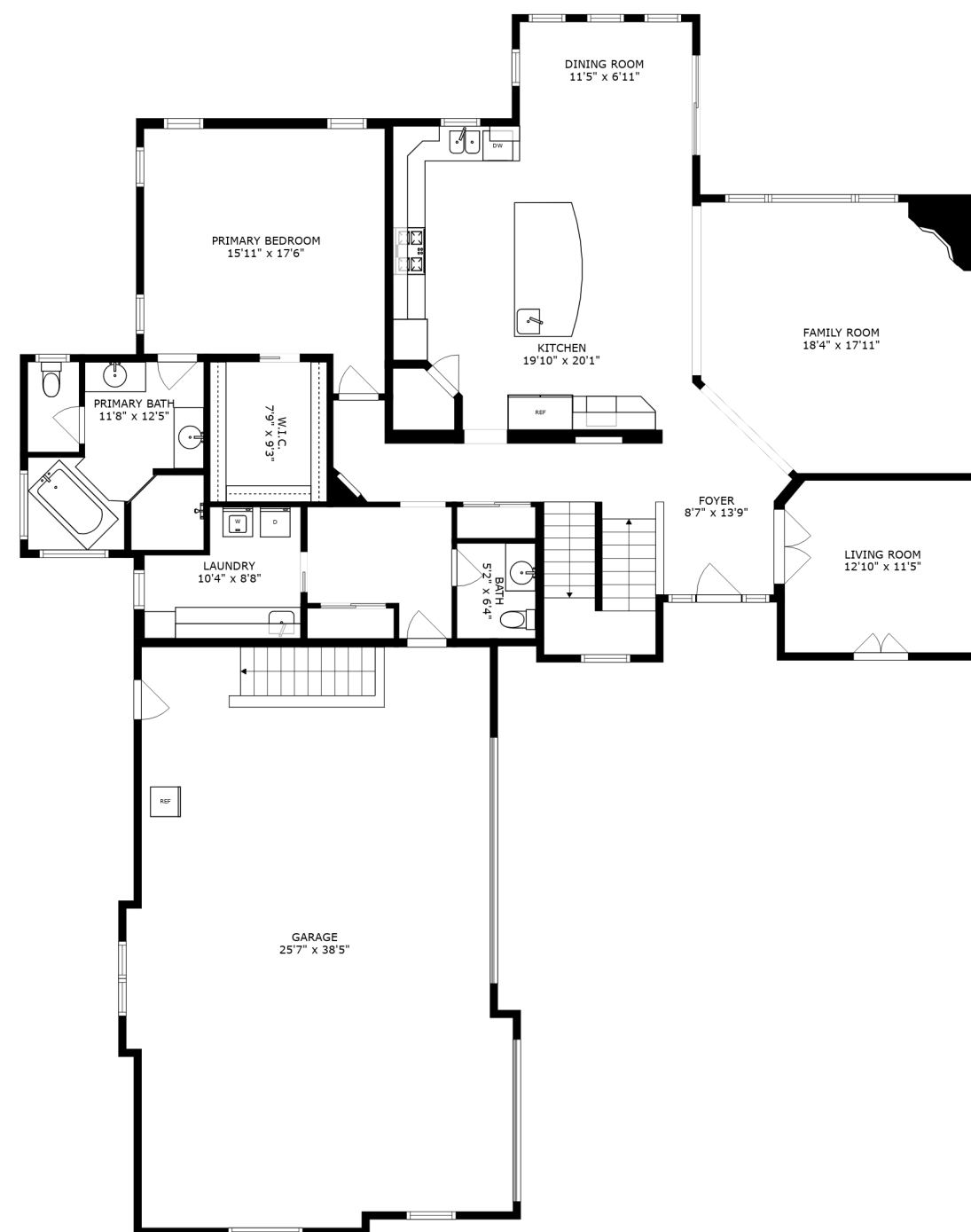
FLOOR 2
