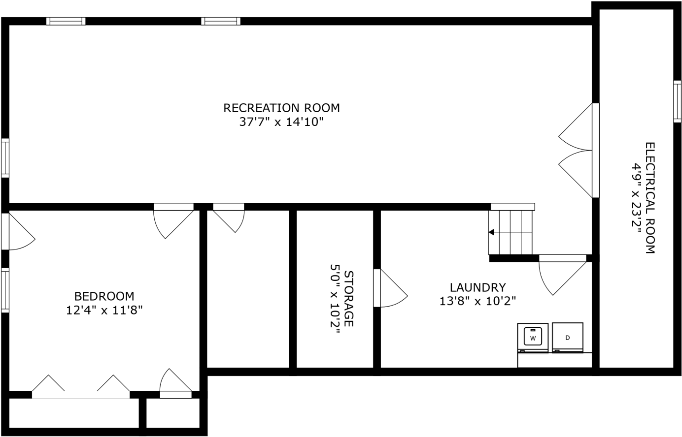
FLOOR 2
