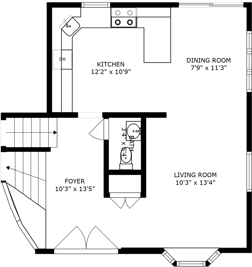
FLOOR 2
