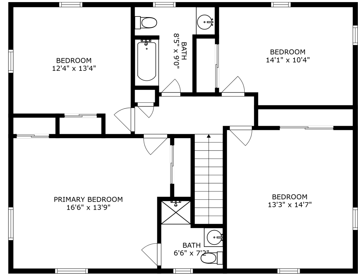
FLOOR 3
