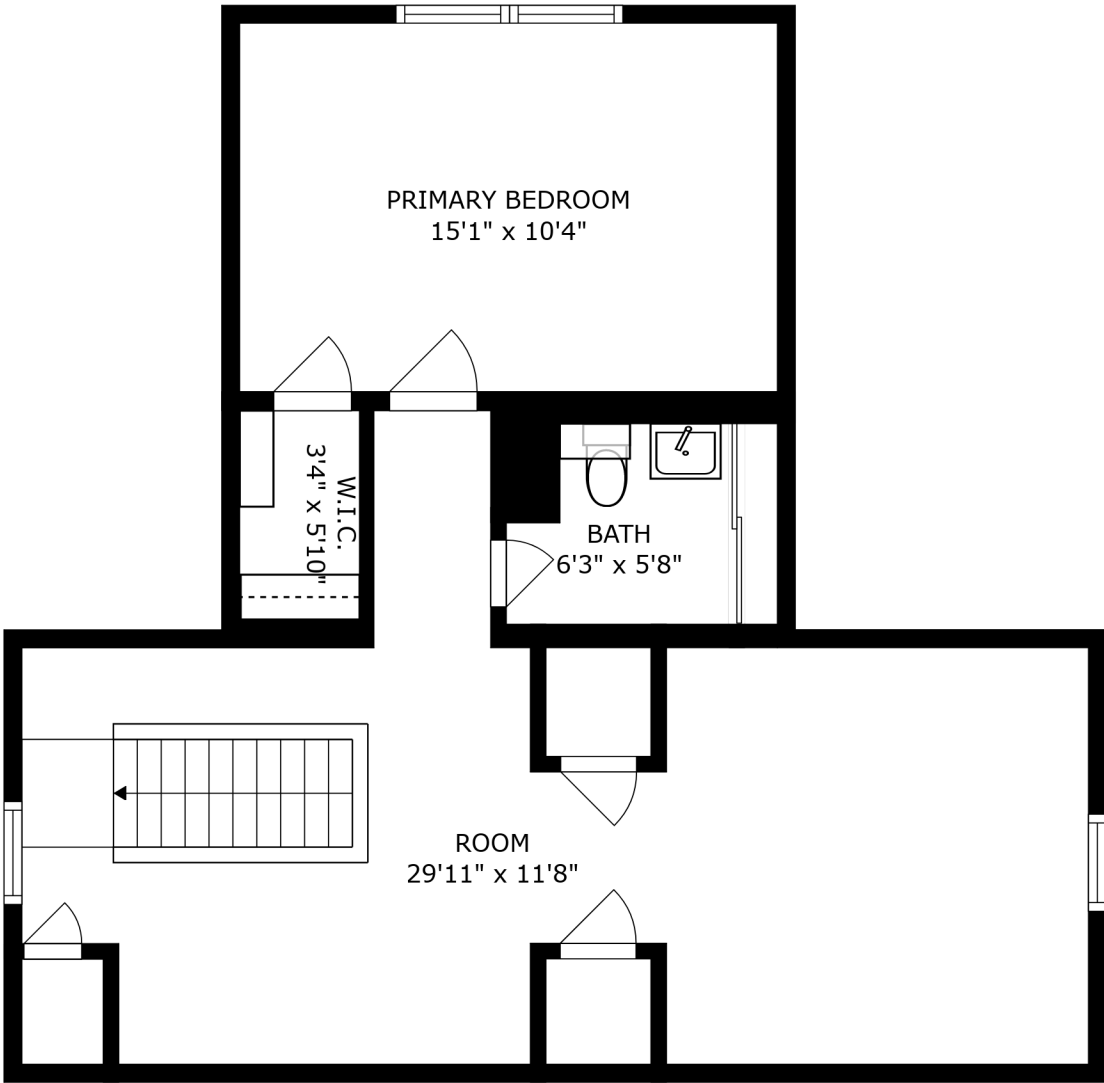
FLOOR 3
