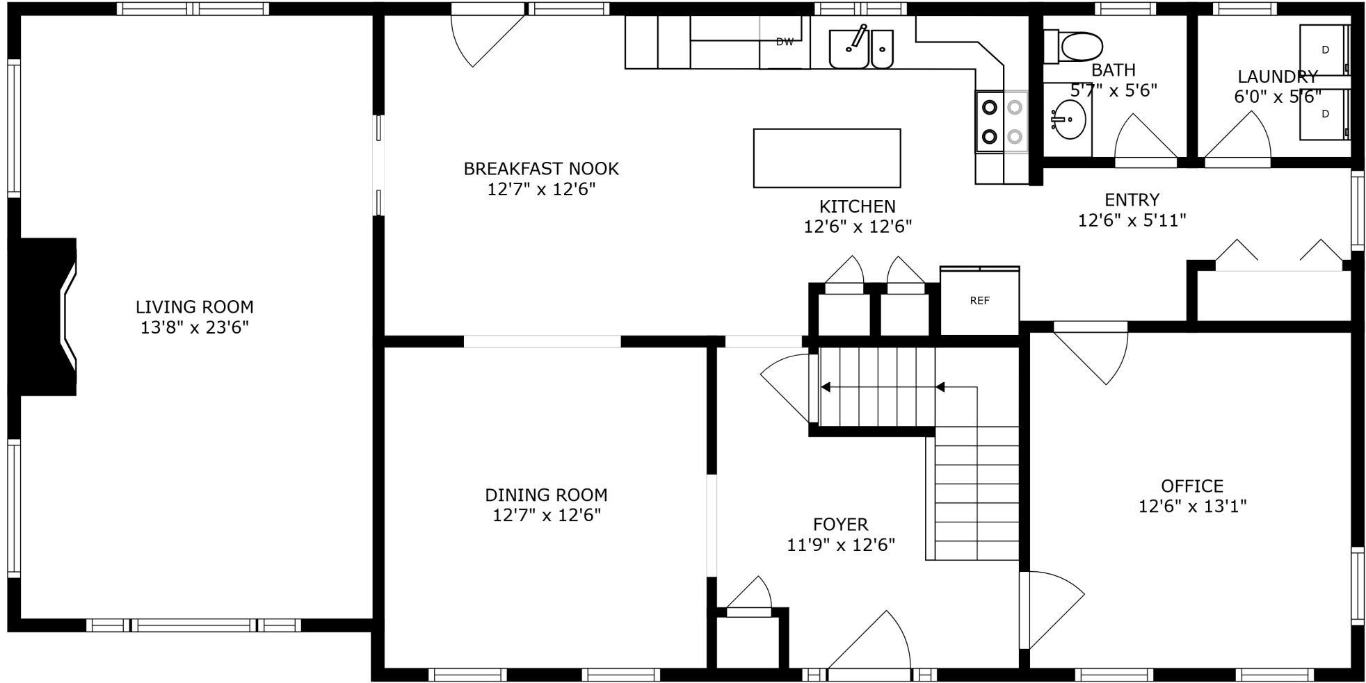
FLOOR 2
