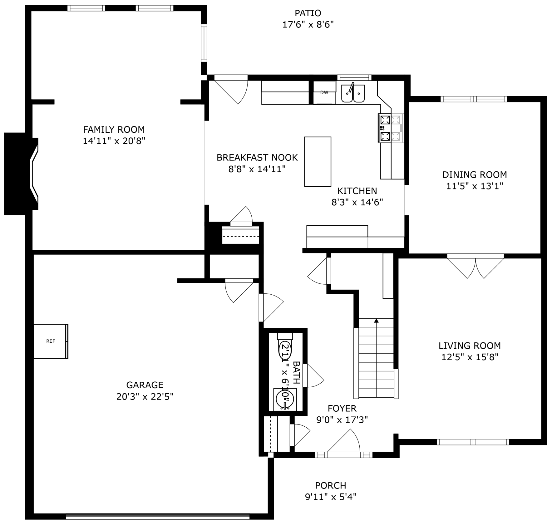
FLOOR 1
