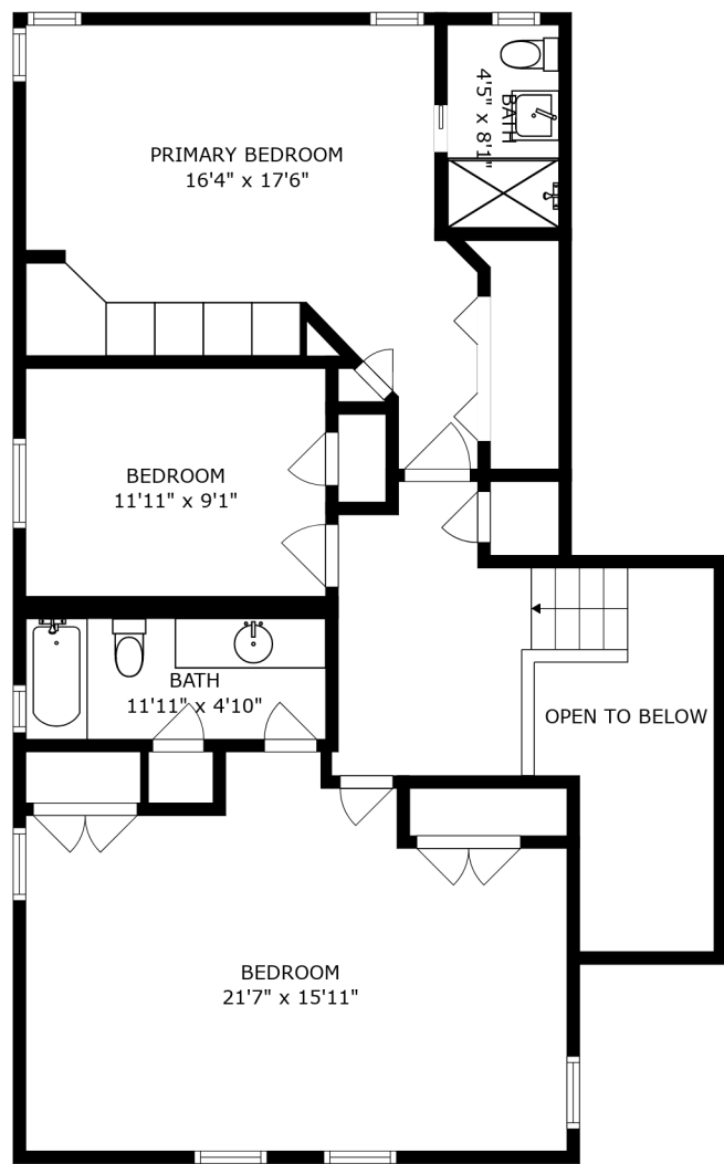
FLOOR 4
